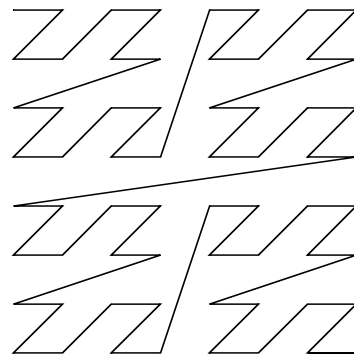
Morton (Z-Curve)
