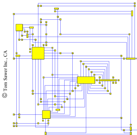
Orthogonal Graph
