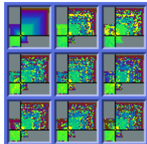
Axes Technique
