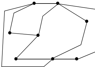
Polyline Drawing
