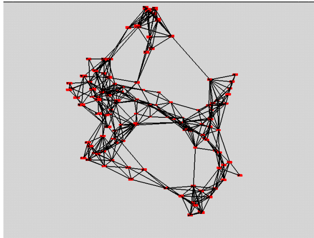
Cluster-Optimized 3D-Graph
