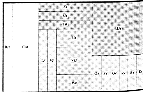
Tree-Map
