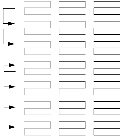
line-by-line loop
