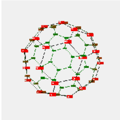
Ball-like Graph
