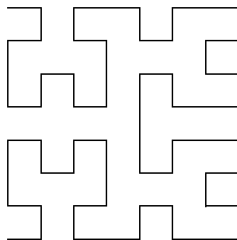
Peano-Hilbert
