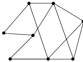
Straight-Line Drawing
