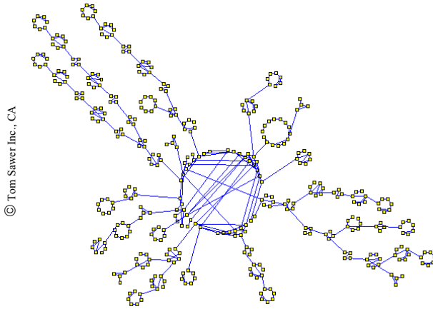
Cluster-Optimized Graph
