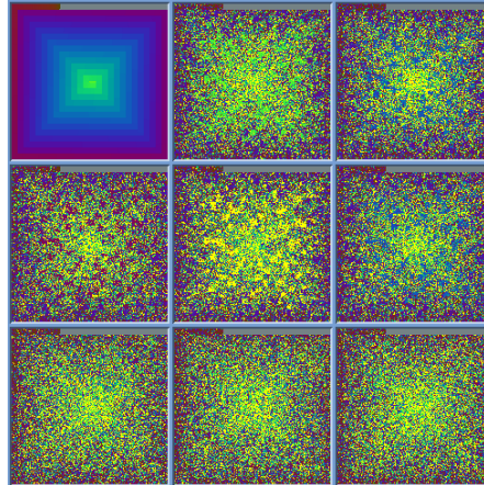
Snake-Spiral Technique
