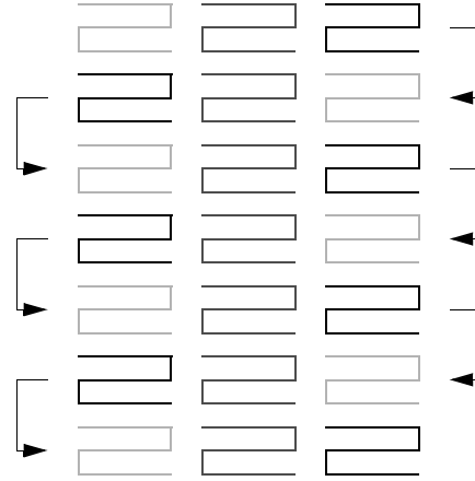
back-and-forth loop
