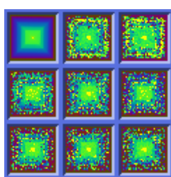
Spiral Technique
