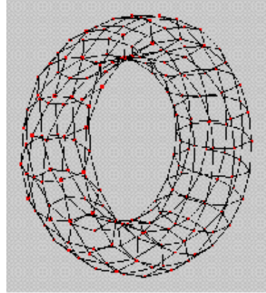
Torus-like Graph
