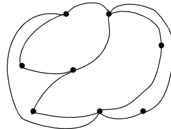
Curved-Line Drawing
