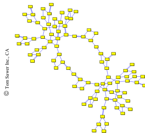
Symmetry-Optimized Graph
