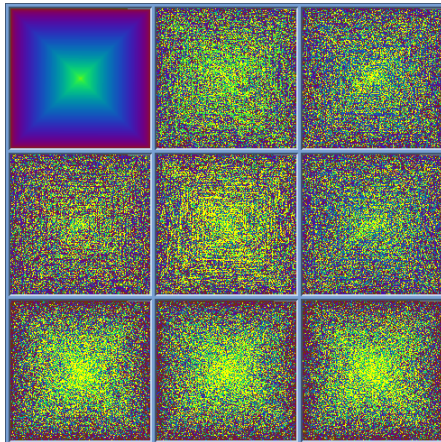
Spiral Technique
