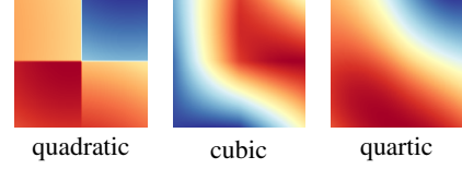
Fig. 4: Quadratic, cubic and quartic B-spline interpolation of the lowest band. Vorticity is color-coded showing discontinuities for lower-order interpolations that negatively affect the flow simulation.
