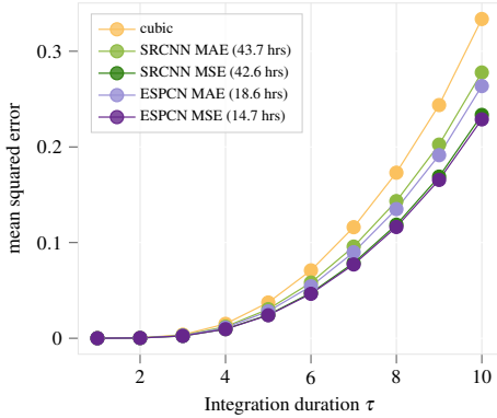
Fig. 9: Quantitative comparison of SRCNN and ESPCN for varying integration durations at 2\times upsampling. ESPCN performed better by a small margin. The required training time is in brackets.
