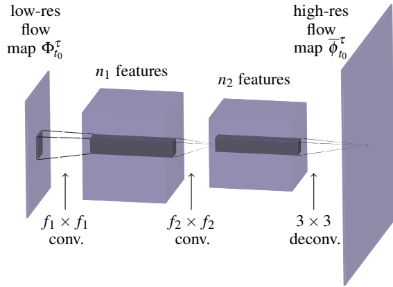
Fig. 5: The ESPCN architecture consists of two convolutional and one deconvolutional layer. A low-resolution flow map goes in and a high resolution flow map is predicted. The convolutional layers have filter size f_1 and f_2 , and compute n_1 and n_2 feature maps, respectively.
