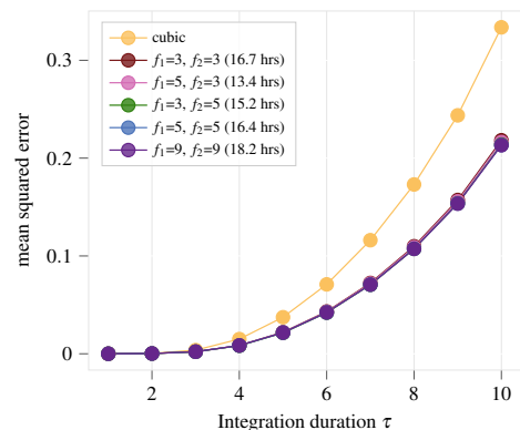
Fig. 7: Study of the filter sizes f_1 and f_2 of the two convolutional layers of ESPCN for a fixed number of features n_1 = n_2 = 64 per layer. The filter size has a marginal effect on the residual, but affects the training time (in brackets) by a few hours.
