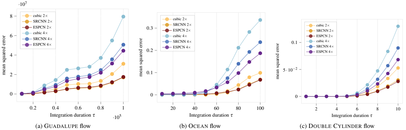
Fig. 13: Error plots of real-world data for varying integration durations with up-scaling factor 2\times and 4\times . Compared to the cubic baseline, SRCNN reduced the error residuals by 44.8% (GUADALUPE), 30.6% (OCEAN) and 42.4% (DOUBLE CYLINDER), whereas ESPCN reduced the error residuals by 43.5% (GUADALUPE), 31.7% (OCEAN) and 47.2% (DOUBLE CYLINDER) at \tau = 10 . For 4\times up-sampling, SRCNN reduced the error residuals by 36.3% (FLOW #2000), 29.6% (BOUSSINESQ) and 30.9% (CYLINDER), whereas ESPCN reduced the error residuals by 44.0% (FLOW #2000), 44.4% (BOUSSINESQ) and 47.6% (CYLINDER) at \tau = 10 .
