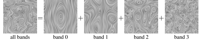
Fig. 3: Wavelet noise-based construction of a random vector field \mathbf{u}(\mathbf{x}) , following Kolmogorov’s energy spectrum. Note that each band \mathbf{w}(\mathbf{x}) is periodic and uses a different random seed.
