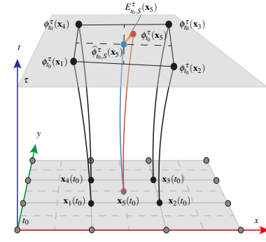
Fig. 2: Space-time visualization of a flow map interpolation from flow maps released from a 4 \times 4 grid at time t_0 in a 2D flow. For seed point \mathbf{x}_5 , the flow map is interpolated from grid vertices \mathbf{x}_1 , \mathbf{x}_2 , \mathbf{x}_3 and \mathbf{x}_4 , resulting in estimate \hat{\phi}_{t_0,S}^\tau(\mathbf{x}_5) (blue), which entails an interpolation error E_{t_0,S}^\tau(\mathbf{x}_5) (orange), compared to the ground truth \phi_{t_0}^\tau(\mathbf{x}_5) (red).
