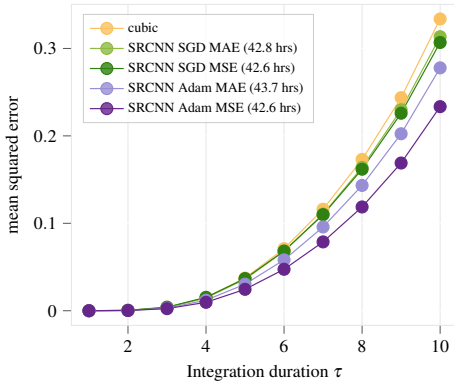
Fig. 8: Hyperparameter adjustment for SRCNN at an upsampling factor of k = 2 . We examine the performance of the stochastic gradient descent and the Adam optimizer, and we explore the choice of the loss function (MSE vs MAE). MSE with Adam optimizer performed best. The required training time is stated in brackets.
