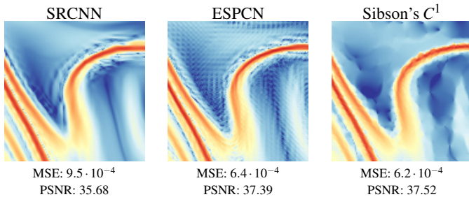
Fig. 14: Comparison of \times 4 up-sampling with adaptive flow map sampling using Sibson’s C^1 continuous interpolation [4] with 128 \times 128 samples. In this example we show the FTLE of close-ups of the flow #2000 for \tau = 3 . Networks with regular grid inputs are less efficient especially in regions without FTLE ridges.
