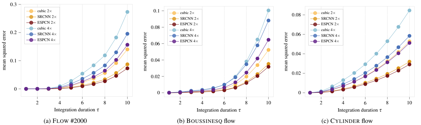
Fig. 11: Error plots of real-world data for varying integration durations with up-scaling factor 2\times and 4\times . Compared to the cubic baseline at 2\times upsampling, SRCNN reduced the error residuals by 37.8% (FLOW #2000), 32.7% (BOUSSINESQ) and 39.4% (CYLINDER), whereas ESPCN reduced the error residuals by 47.9% (FLOW #2000), 39.4% (BOUSSINESQ) and 44.9% (CYLINDER) at \tau = 10 . For 4\times upsampling, SRCNN reduced the error residuals by 28.6% (FLOW #2000), 12.2% (BOUSSINESQ) and 30.9% (CYLINDER), whereas ESPCN reduced the error residuals by 42.9% (FLOW #2000), 35.6% (BOUSSINESQ) and 39.4% (CYLINDER) at \tau = 10 .
