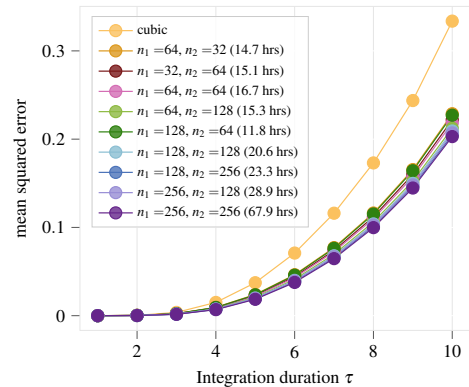
Fig. 6: Varying the number of features n_1 and n_2 in the two convolutional layers of ESPCN for a fixed filter size of f_1 = f_2 = 3 . Growing the feature size further does not pay off in terms of the remaining error residual compared to the increasing training time (in brackets).
