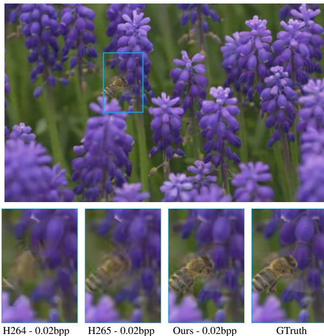
Figure 1: Learning based video compression. Compared to existing video codecs, our method achieves better results at a similar or lower bit rate. Less visual artifacts are present and colors are closer to the original (best viewed on screen).
