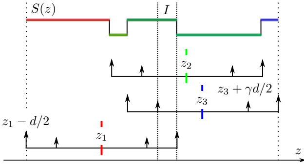
Figure 4: This figure illustrates the algorithm for determining the replacement colors. Three fragments are shown with their compositing windows ( \pm d ) and box filter windows ( \pm \gamma d ). The stroke order is z_1, z_3, z_2 . During the integration, the contribution of the interval I is added to the replacement colors of fragments z_2 and z_3 . The vertical separation is used only to make the illustration less cluttered.
