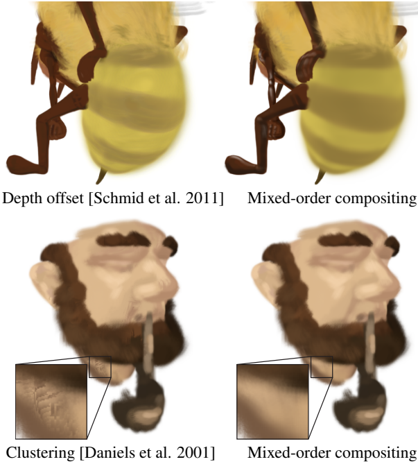
Figure 6: A comparison between existing methods and mixed-order compositing. The optimal parameters have been manually chosen for each algorithm. The left column shows artifacts on the bee’s limbs and abdomen and on the captain’s neck, mouth, and nose regions. These images are best viewed zoomed in. As our video demonstrates, all of these artifacts are time-varying.
