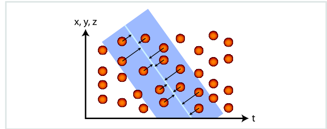
Fig. 4 Samples of the video hypervolume (orange) are intersected with the hyperslice (blue) and projected onto its center plane.
