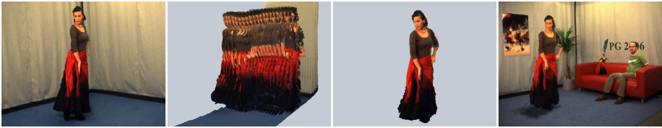
Fig. 2 Our interactive 3D video editing combines the advantages of 2D video editing with depth-enhanced 3D video streams. From left to right: Interpolated view of the 3D video input data; hyperslicing to reveal the time domain where selection and editing is intuitive and easily performed; cutout of a 3D video object; composite 3D video with additional 2D and 3D objects, new background and shadow mapping.
