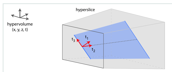
Fig. 5 Non-orthogonal slices are generated by calculating the required rotation matrix simply from a line drawn onto the screen.
