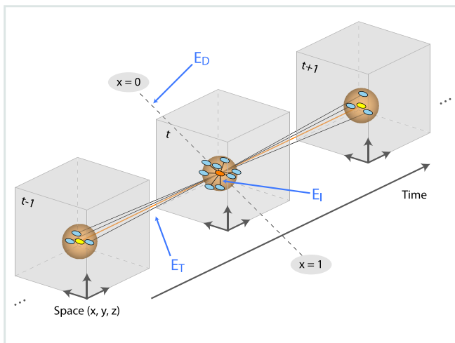
Fig. 7 When constructing the 4D graph, any data sample or data region contributes to the graph according to intra-frame and inter-frame neighborhoods and energies, as well as to virtual nodes with data energies.
